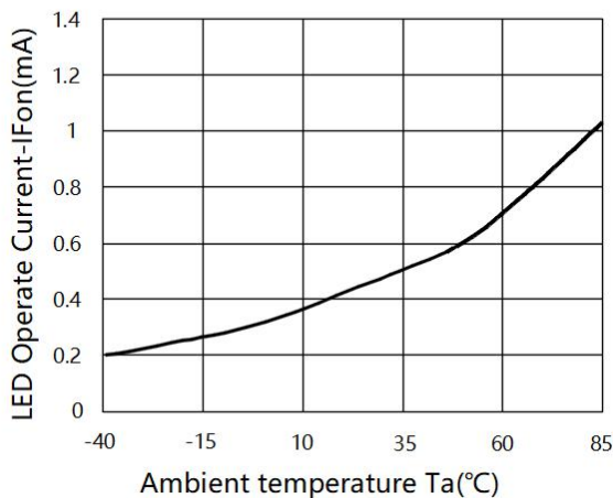
Fig.5 LED Operate Current I_{Fon} (mA) vs Ambient Temperature
