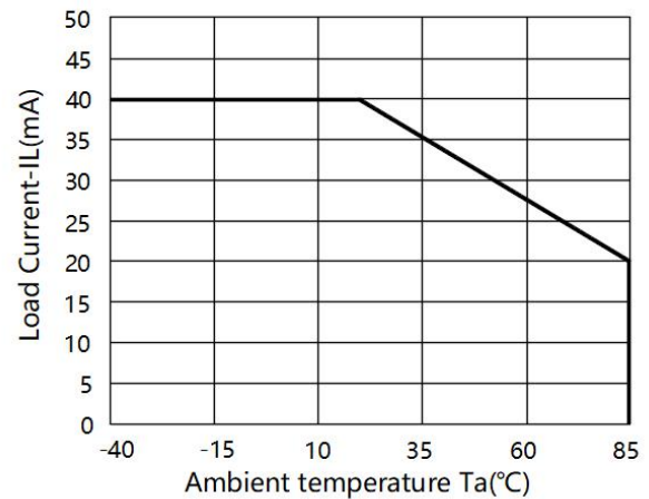
Fig.4 Load Current vs Ambient temperature
