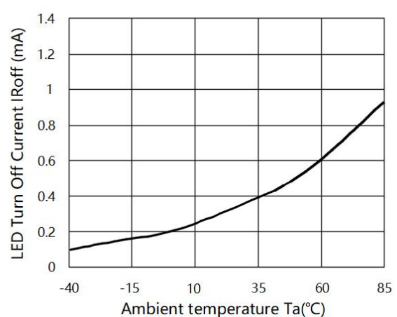
Fig.6 LED Turn Off Current I_{Roff} (mA) vs Ambient Temperature
