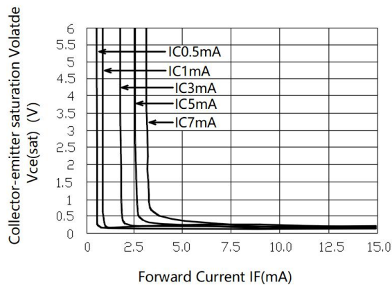
Fig.9 Collect-emitter Saturation Voltage vs. Forward Current
