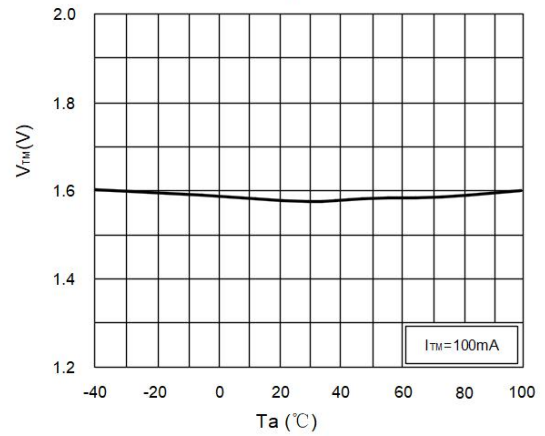
Fig.8 On-state Terminal Voltage vs. Ambient Temperature
