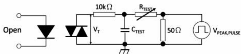
Fig.15 Test Circuits of dv/dt
