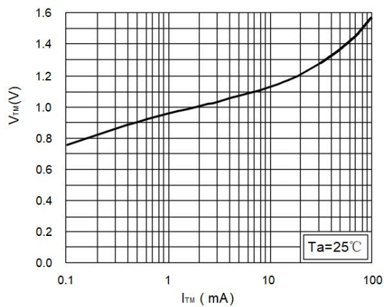
Fig.9 On-state Terminal Voltage vs. On-state Terminal Current
