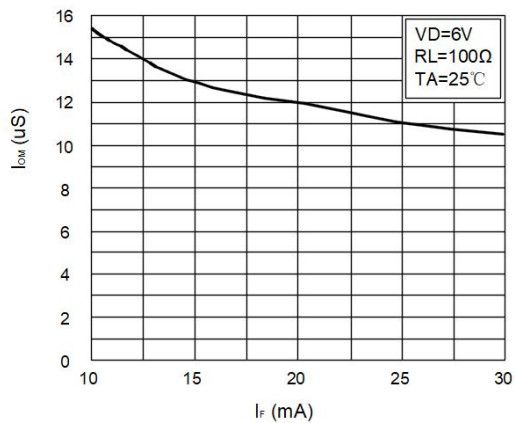
Fig.11 Tun On Time vs. Forward Current
