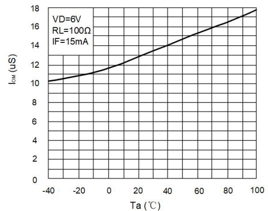
Fig.12 Tun On Time vs. Ambient Temperature
