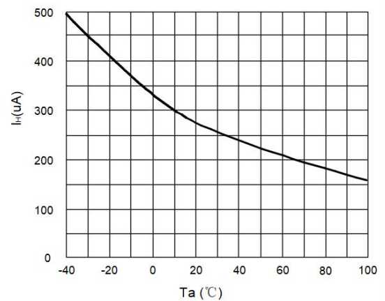
Fig.10 Holding Current vs. Ambient Temperature
