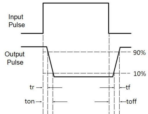
Fig.14 Waveforms of Turn On Time
