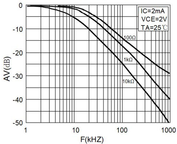
Fig.11 Frequency Response
