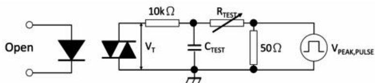
Fig.17 Test Circuits of dv/dt
