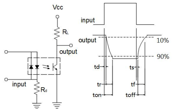
Fig.10 Switching Time Test Circuit & Waveforms
