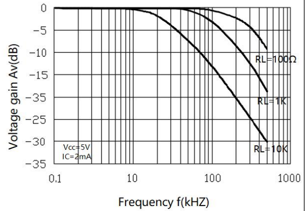
Fig.8 Frequency Response
