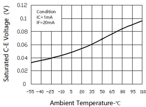
Fig.5 Collector-emitter Saturation Voltage vs. Ambient Temperature
