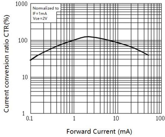
Fig1.Relative Current Transfer Ratio vs. Forward Current
