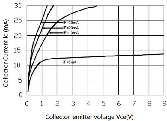
Fig.3 Collector Current vs. Collect-emitter voltage
