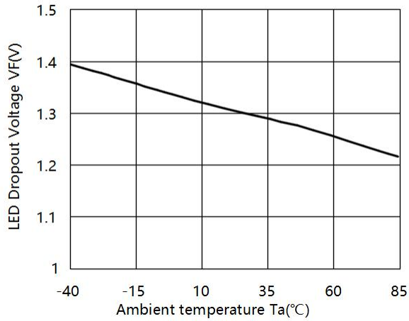
Fig.1 LED Dropout Voltage vs Ambient temperature
