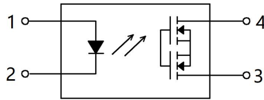
Pin Configuration
