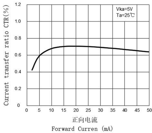
电流传输比CTR与正向电流特性曲线 Current transfer ratio CTR vs. Forward Current
