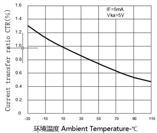
电流传输比CTR与环境温度特性曲线 Current transfer ratio CTR vs.Ambient Temperature
