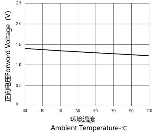
正向电压与环境温度特性曲线 Forward Voltage vs.Ambient Temperature
