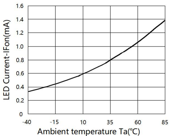
Fig.5 LED Turn On Current vs Ambient Temperature
