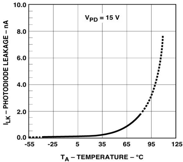
Typical photodiode leakage vs. temperature.
