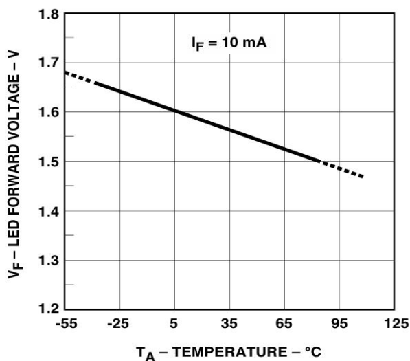
LED forward voltage vs. temperature.
