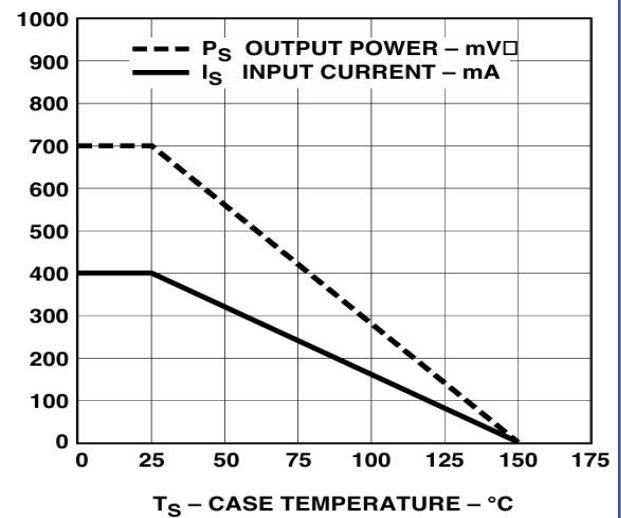
Thermal derating curve dependence of safety limiting value with case temperature
