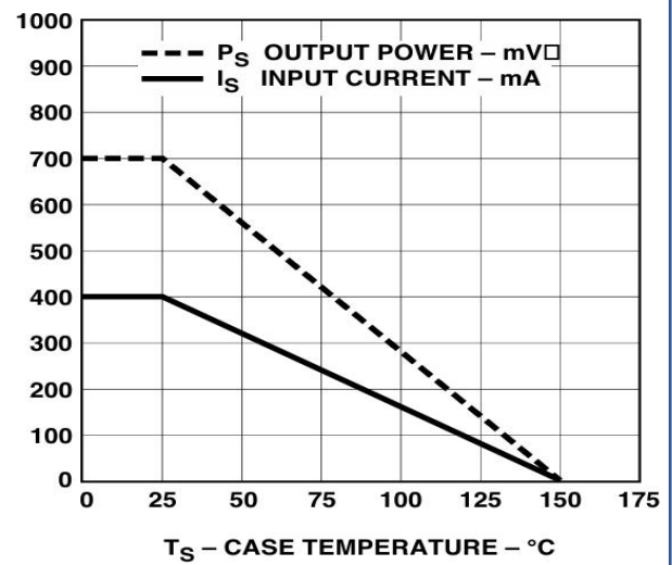
Thermal derating curve dependence of safety limiting value with case temperature
