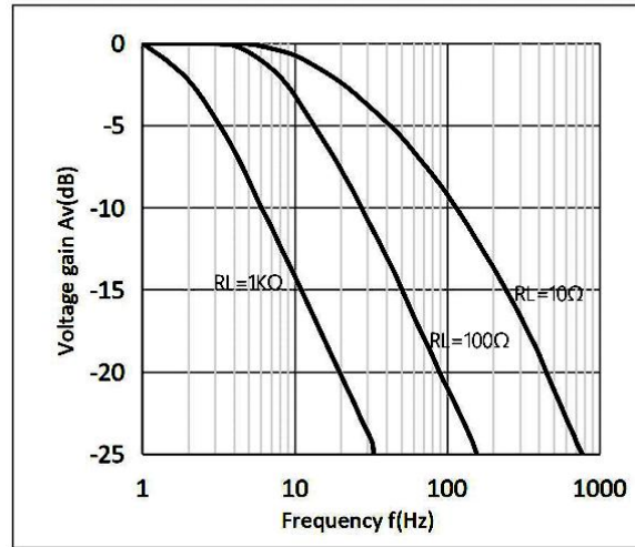
Fig.8 Frequency Response
