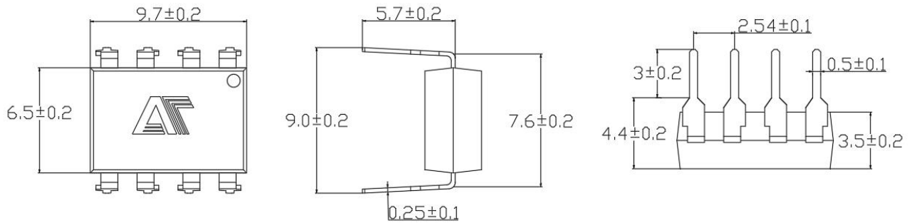
DIP8
