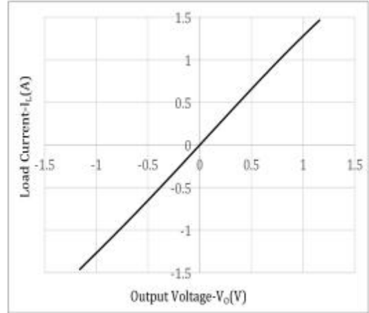
Fig.2 Current vs. Voltage Characteristics Of Output At MOS Portion
